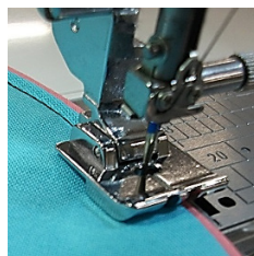
202-489-009 Piping foot (narrow) Max. cord size 3 mm
